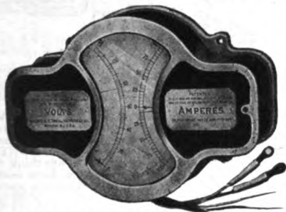
Combination Volt and Ammeter Model 36
